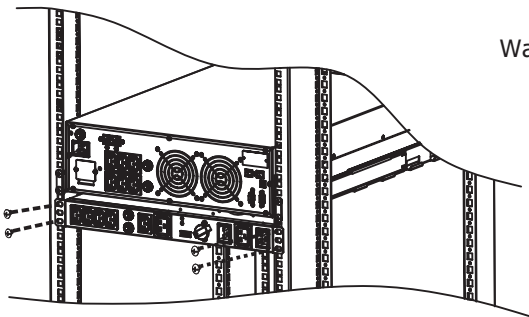
Chart 1: Rack mounting
